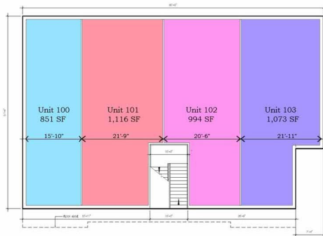
Bldg 1 1st Floor 4,043 SF
