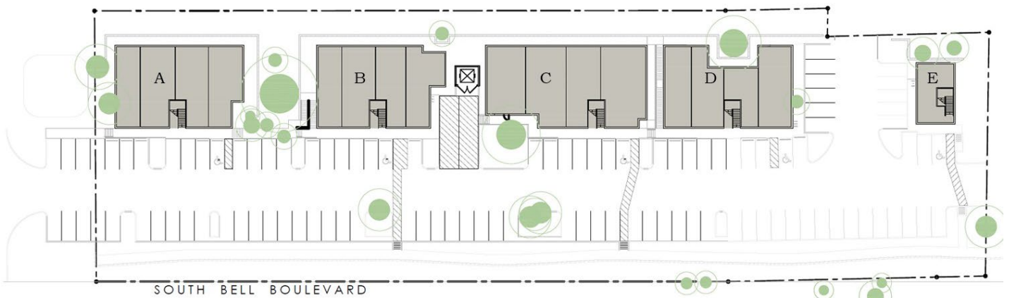
Site Plan GROUND LEVEL 1"=40'-0"
